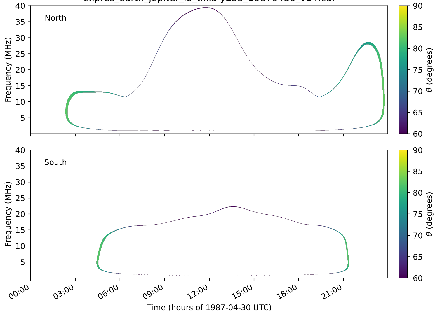
expres_earth_jupiter_io_txka-y235_19870430_v14.cdf
