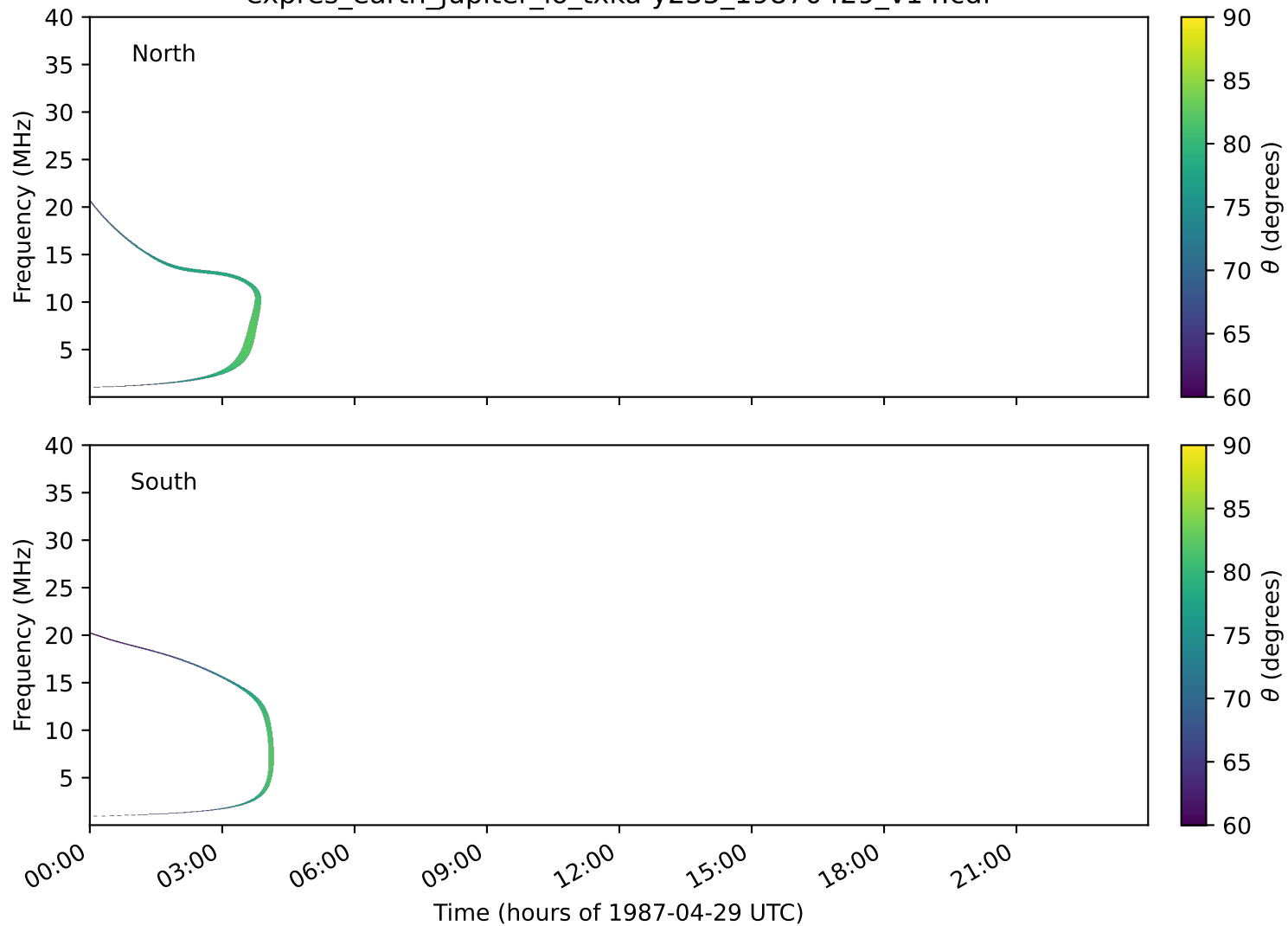
expres_earth_jupiter_io_txka-y235_19870429_v14.cdf
