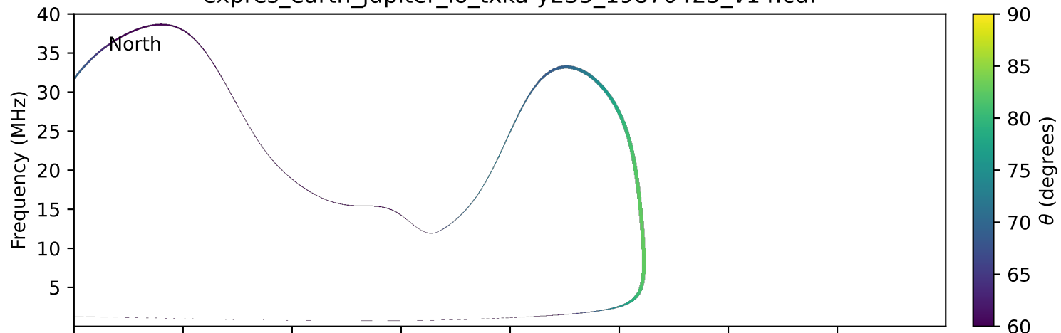
expres_earth_jupiter_io_txka-y235_19870425_v14.cdf
