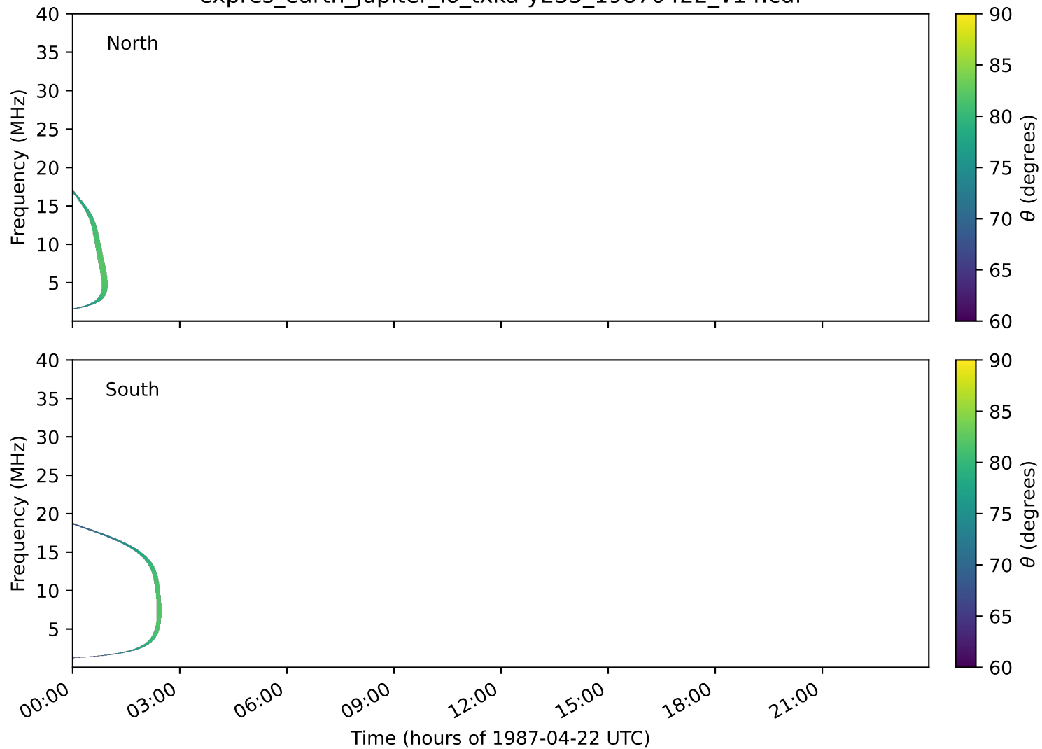
expres_earth_jupiter_io_txka-y235_19870422_v14.cdf
