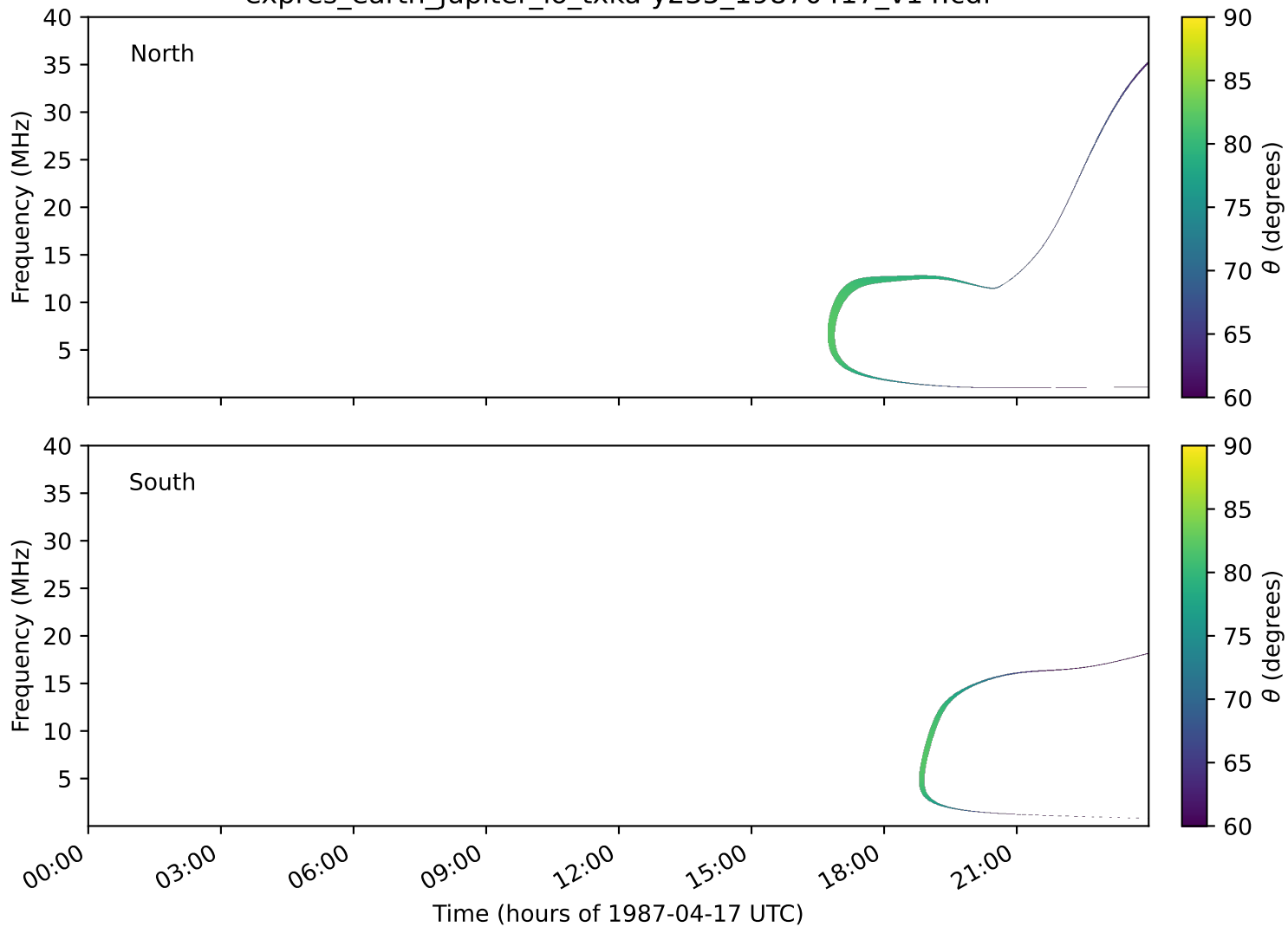
expres_earth_jupiter_io_txka-y235_19870417_v14.cdf
