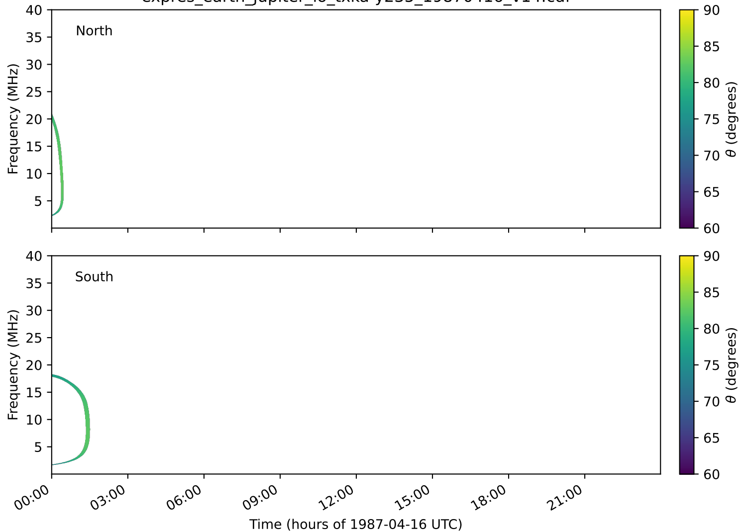
expres_earth_jupiter_io_txka-y235_19870416_v14.cdf
