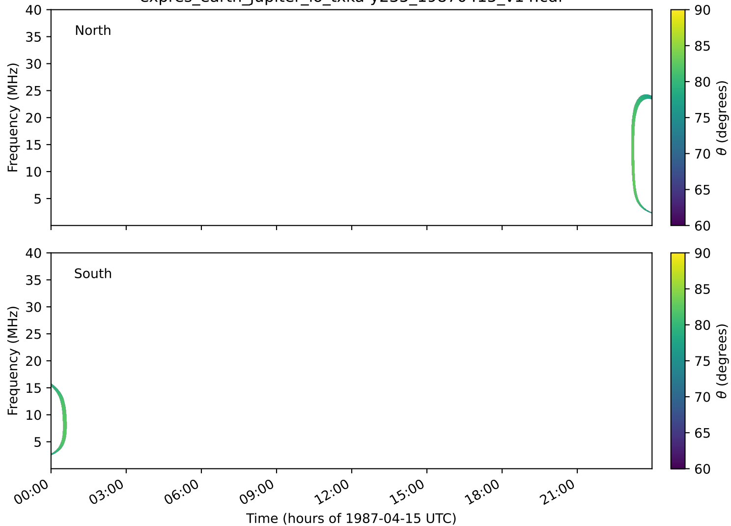
expres_earth_jupiter_io_txka-y235_19870415_v14.cdf
