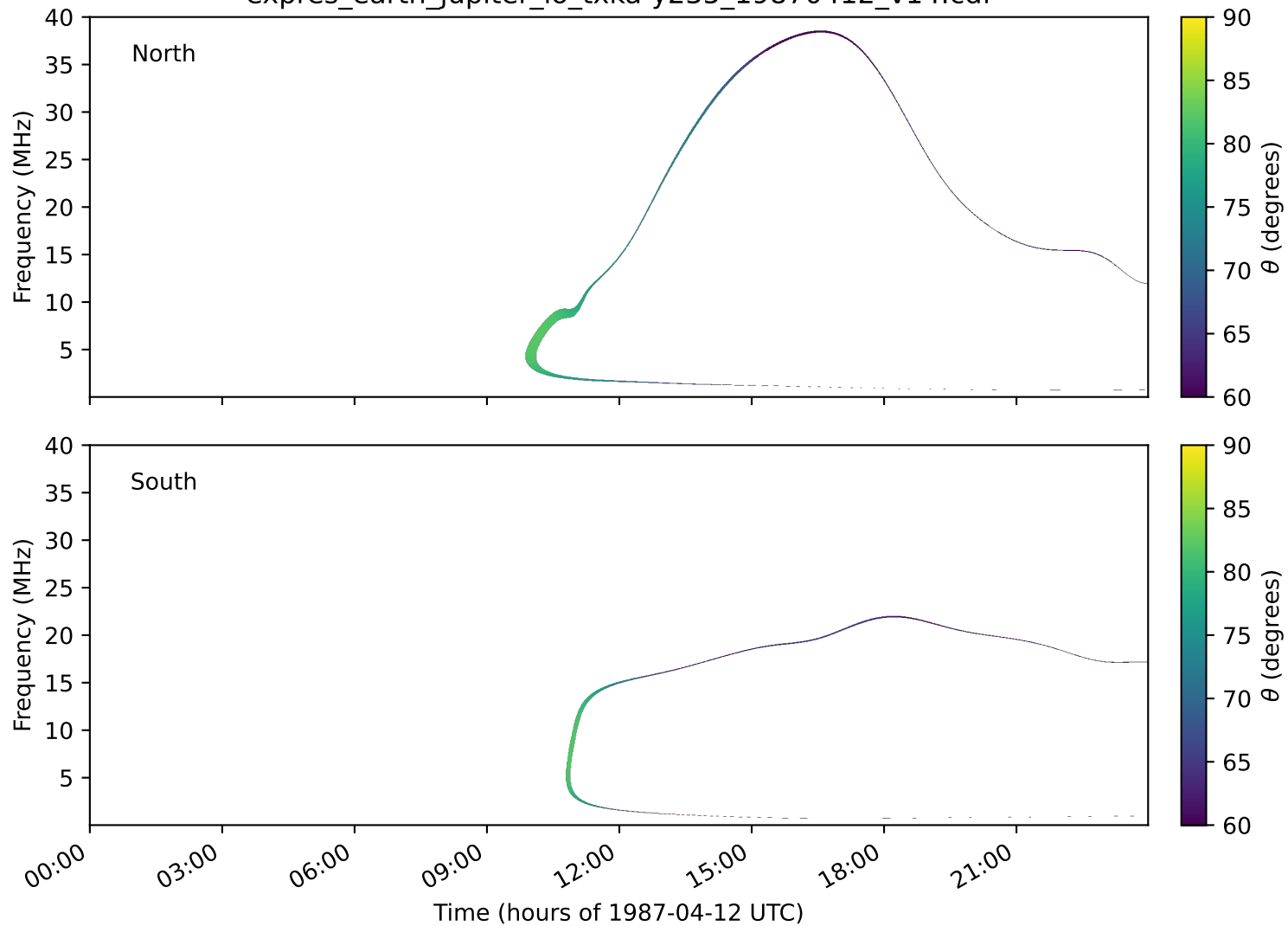
expres_earth_jupiter_io_txka-y235_19870412_v14.cdf
