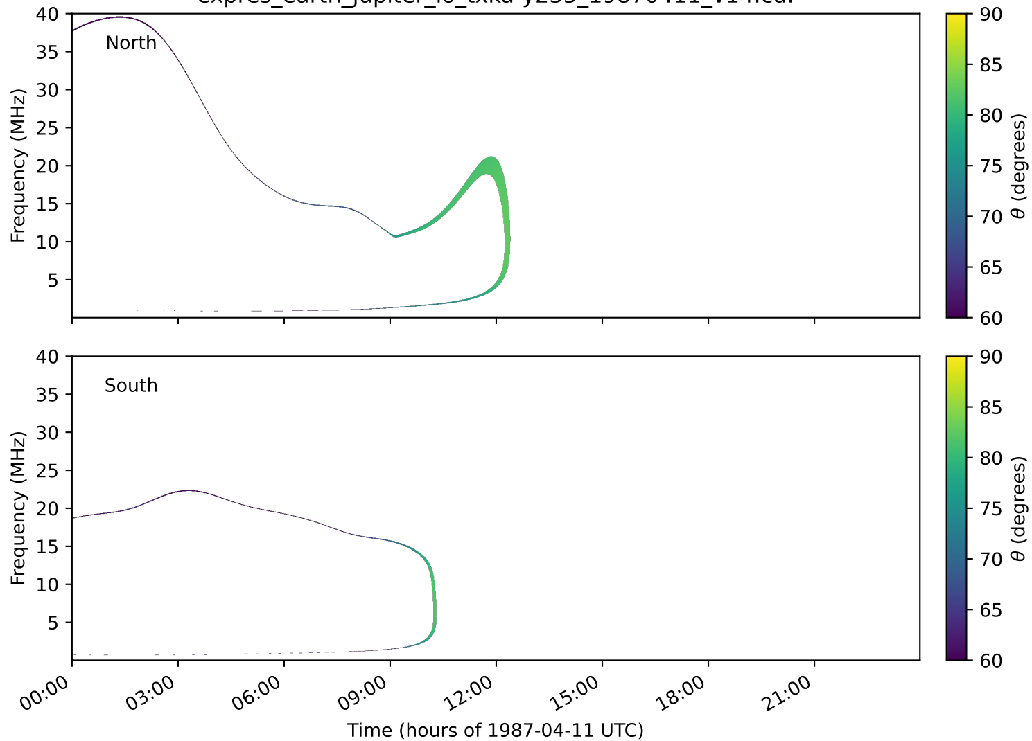
expres_earth_jupiter_io_txka-y235_19870411_v14.cdf
