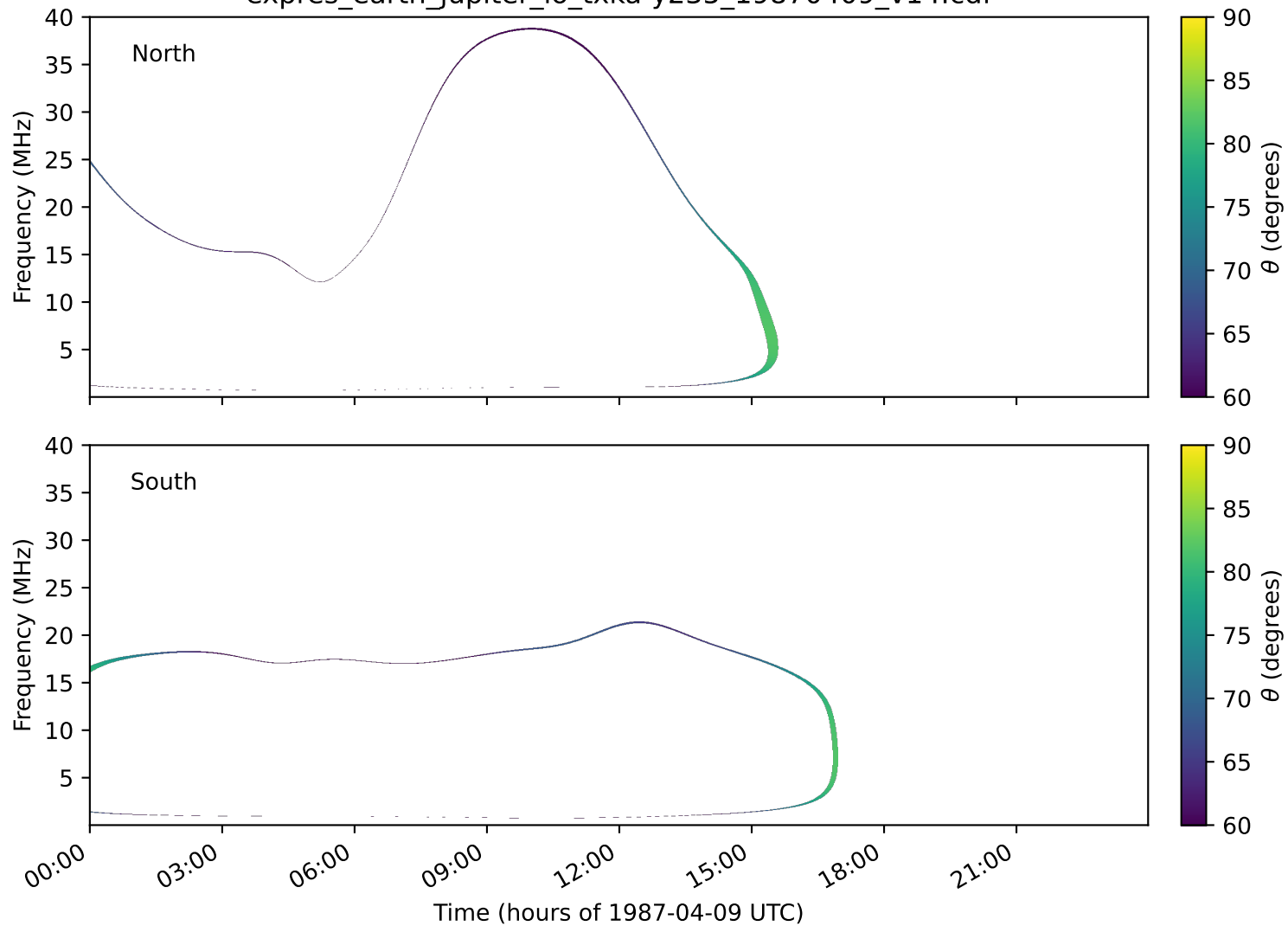
expres_earth_jupiter_io_txka-y235_19870409_v14.cdf
