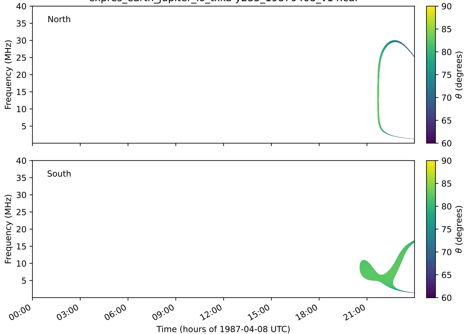
expres_earth_jupiter_io_txka-y235_19870408_v14.cdf
