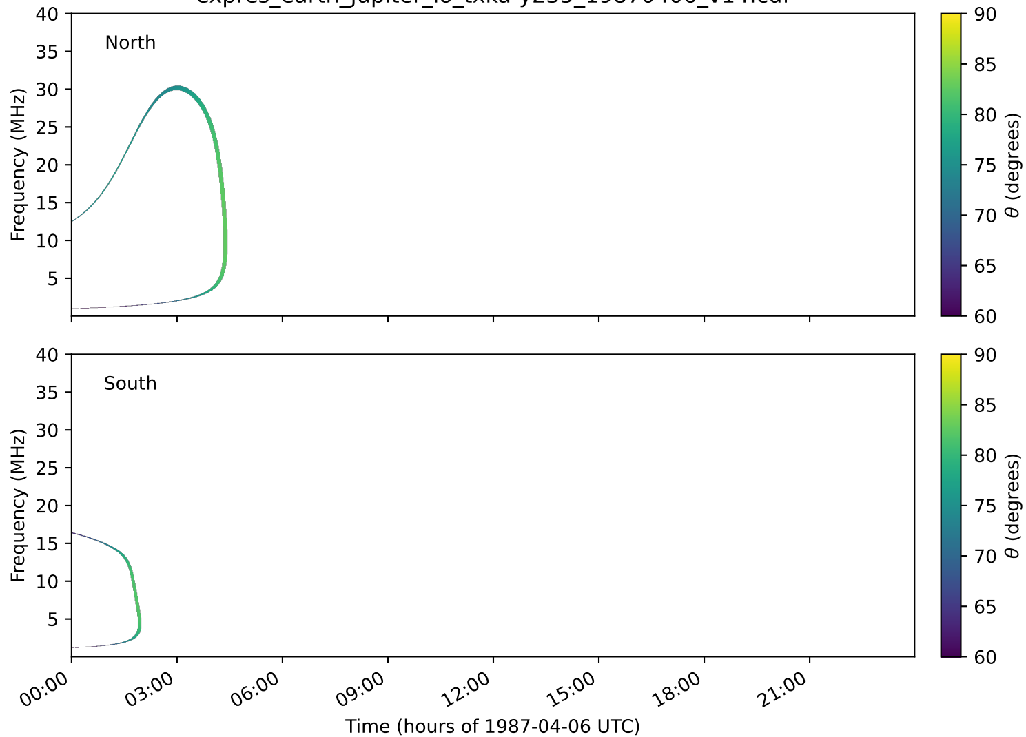
expres_earth_jupiter_io_txka-y235_19870406_v14.cdf
