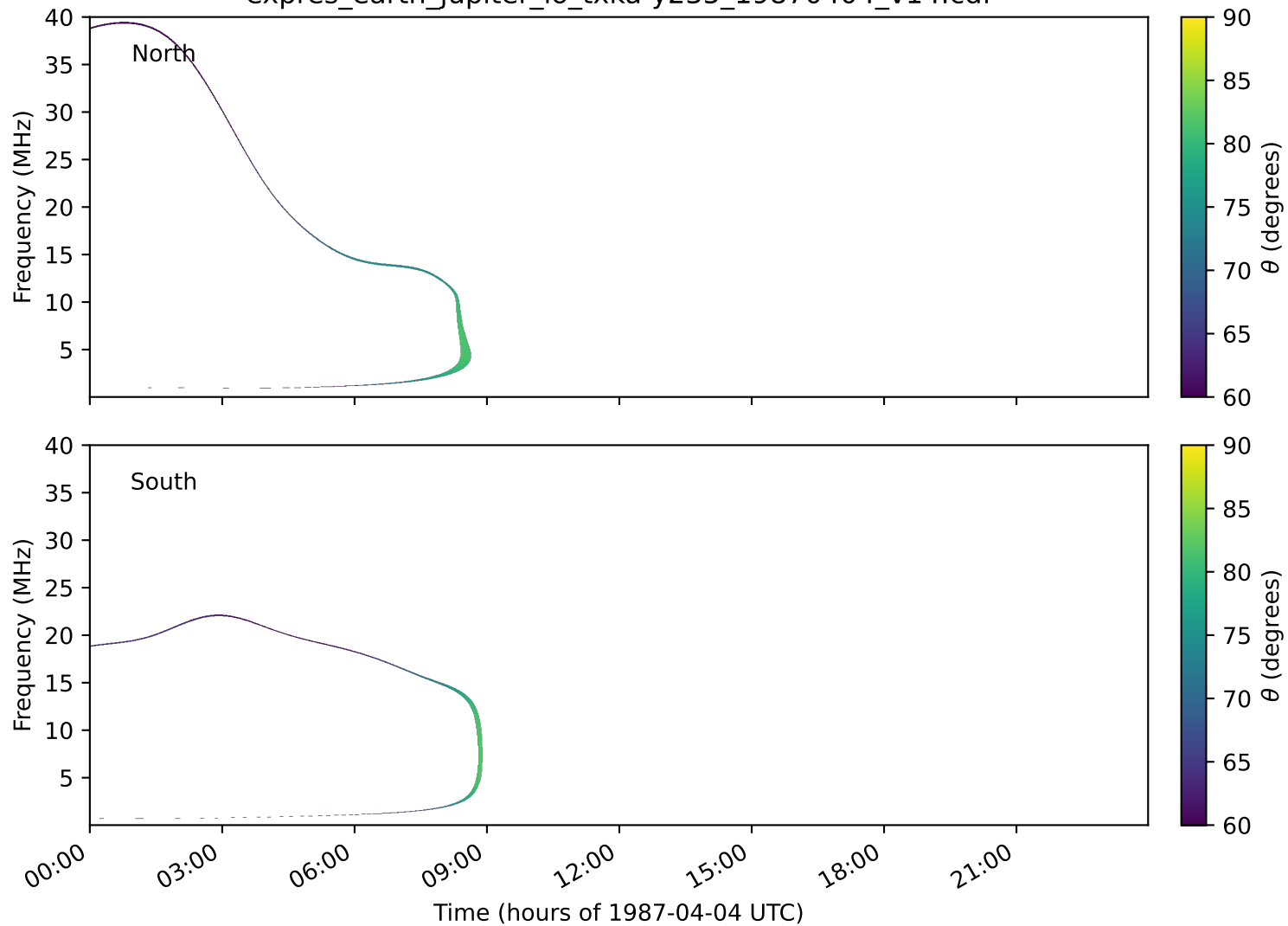
expres_earth_jupiter_io_txka-y235_19870404_v14.cdf
