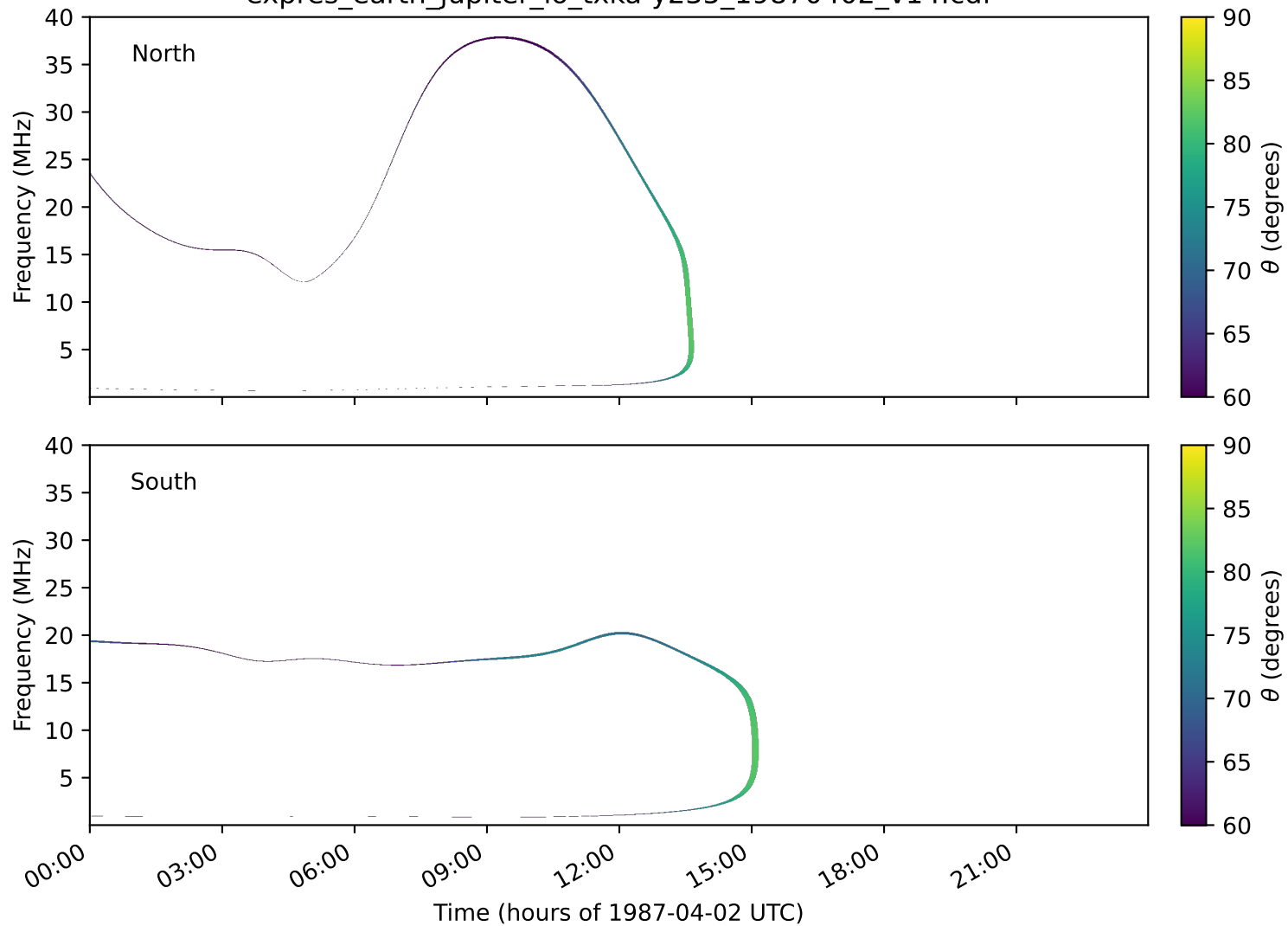
expres_earth_jupiter_io_txka-y235_19870402_v14.cdf
