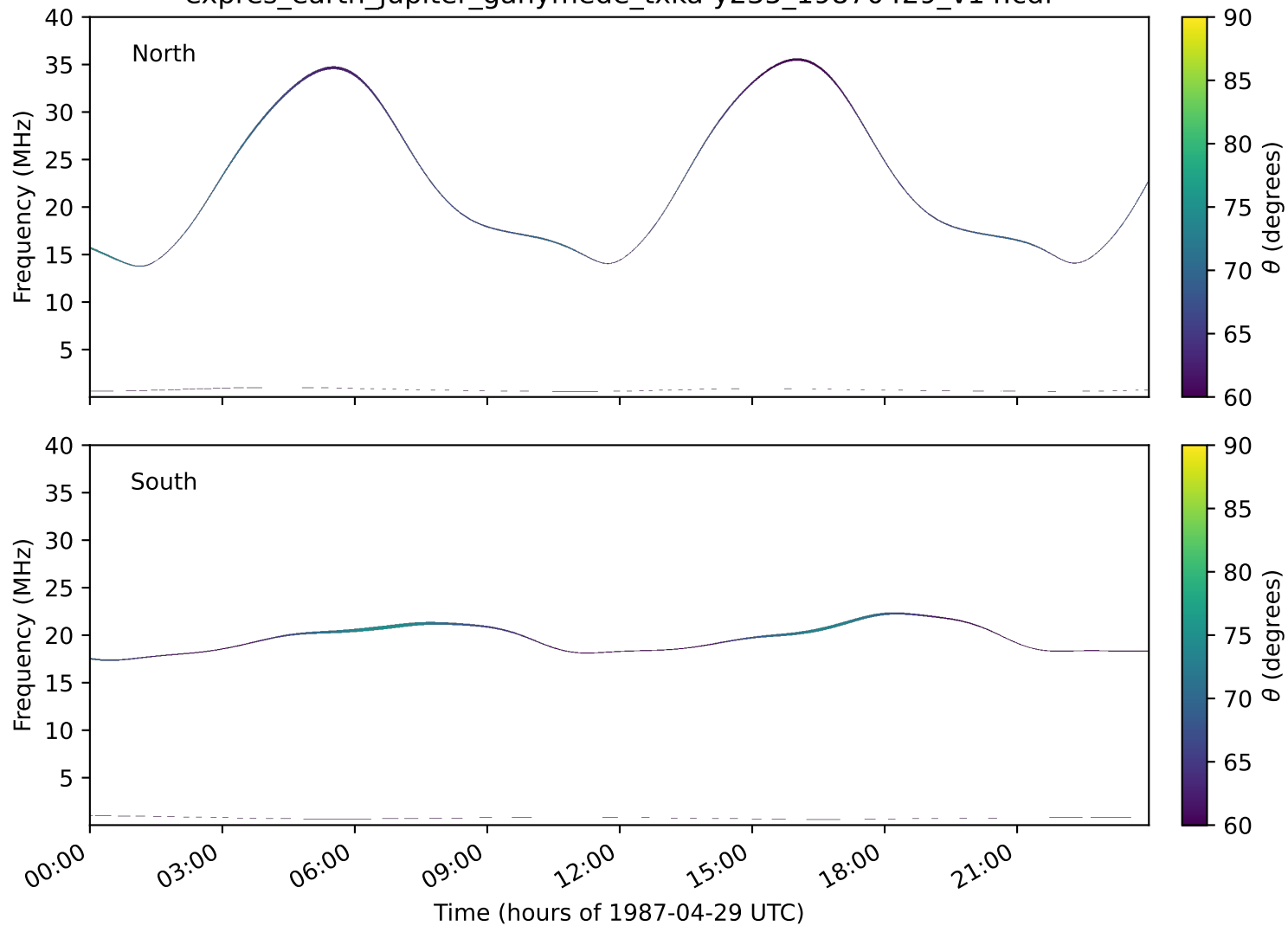
expres_earth_jupiter_ganymede_txka-y235_19870429_v14.cdf
