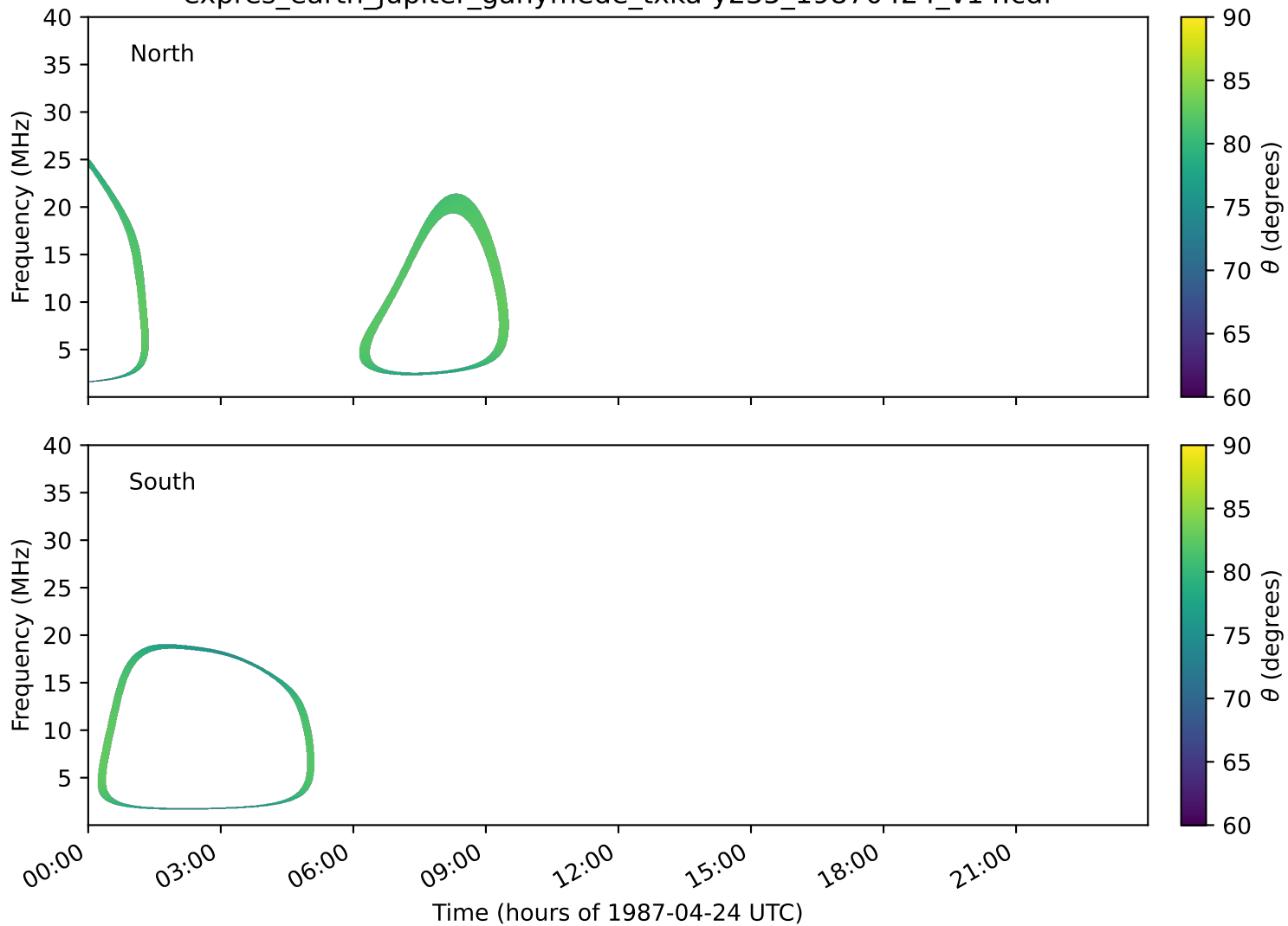
expres_earth_jupiter_ganymede_txka-y235_19870424_v14.cdf
