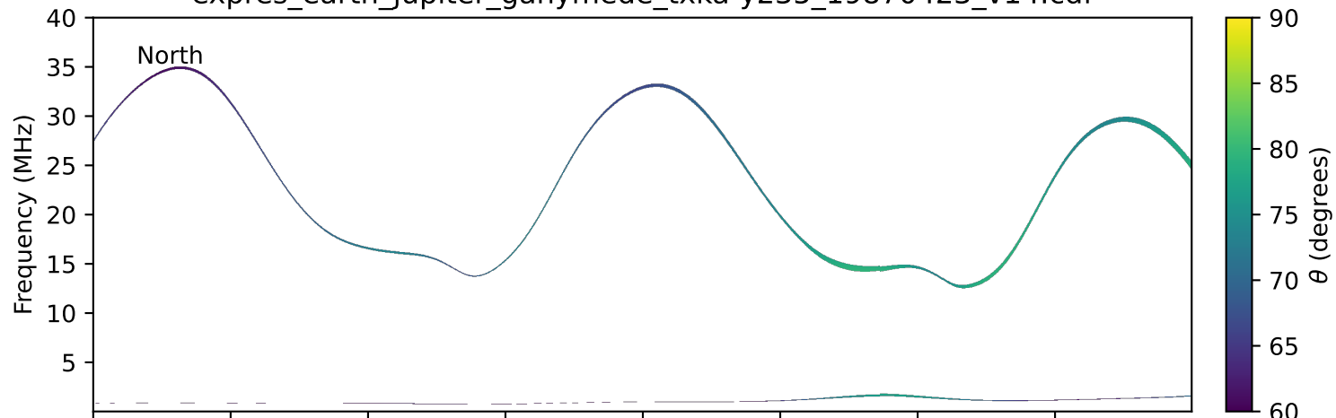
expres_earth_jupiter_ganymede_txka-y235_19870423_v14.cdf
