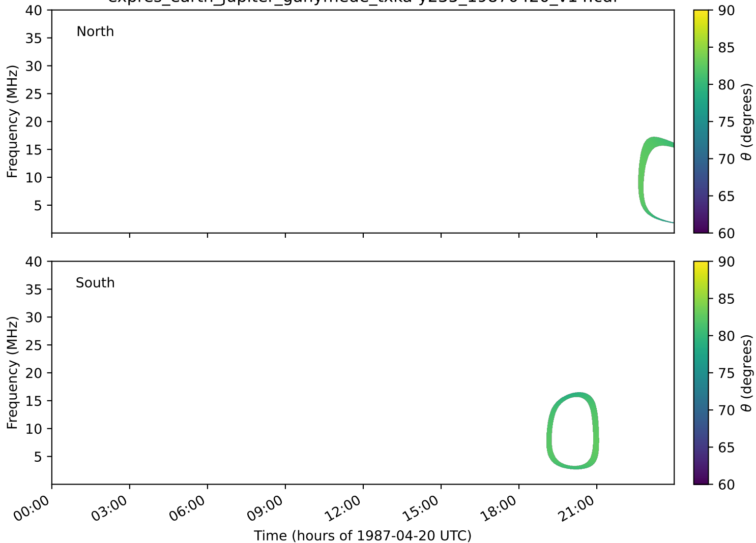
expres_earth_jupiter_ganymede_txka-y235_19870420_v14.cdf
