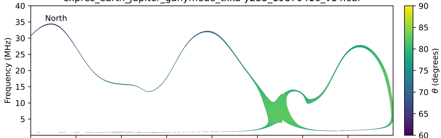
expres_earth_jupiter_ganymede_txka-y235_19870416_v14.cdf
