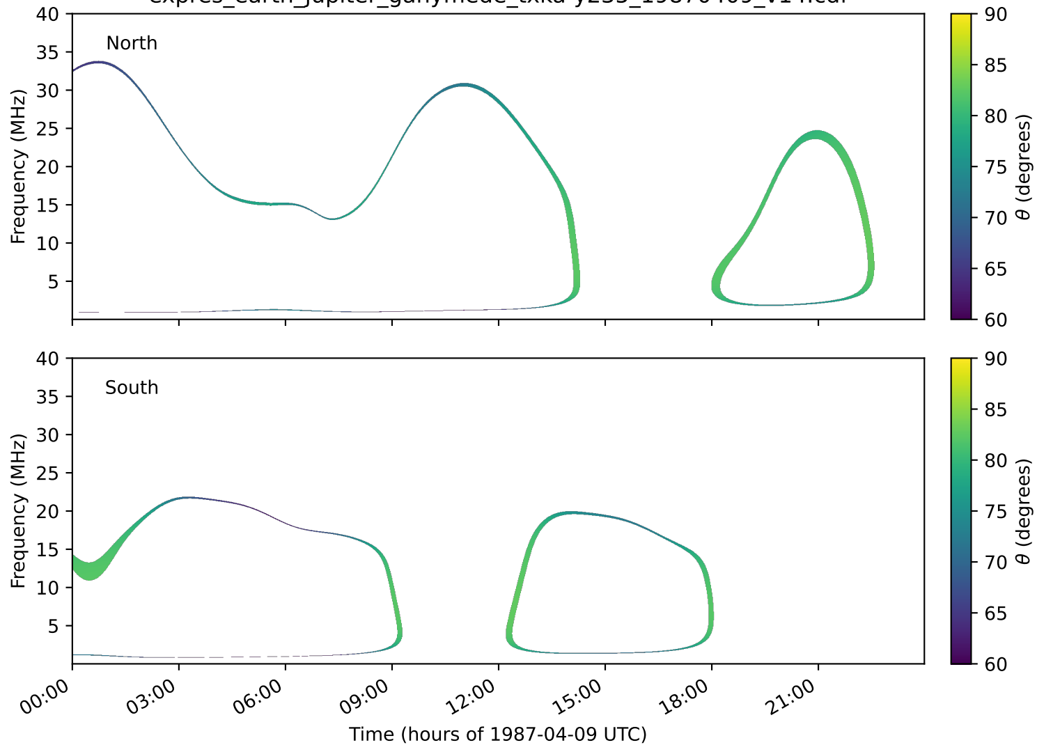
expres_earth_jupiter_ganymede_txka-y235_19870409_v14.cdf
