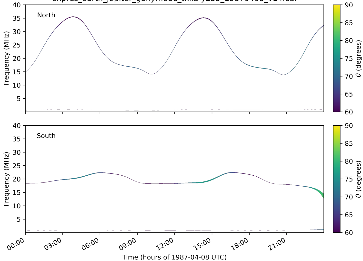
expres_earth_jupiter_ganymede_txka-y235_19870408_v14.cdf
