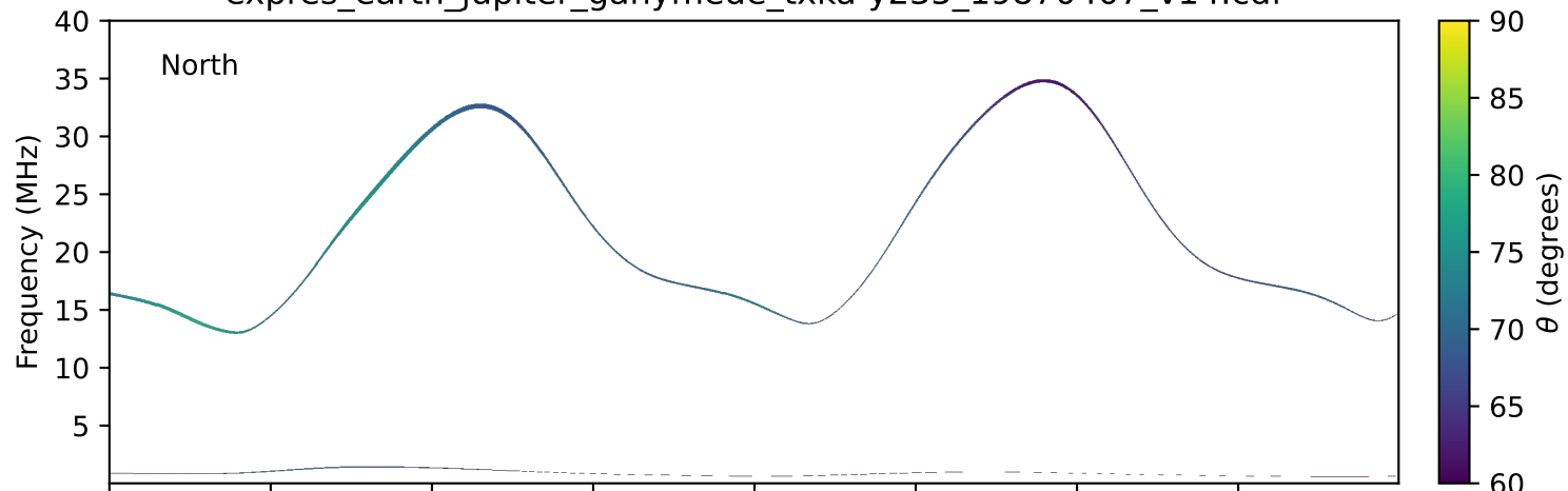
expres_earth_jupiter_ganymede_txka-y235_19870407_v14.cdf
