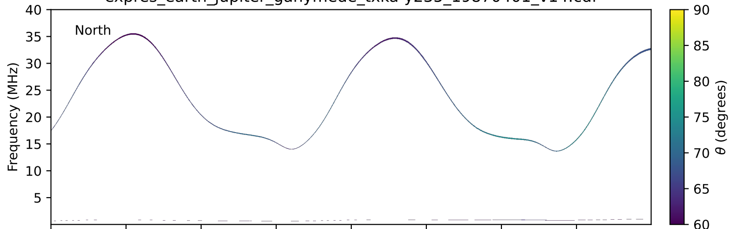
expres_earth_jupiter_ganymede_txka-y235_19870401_v14.cdf
