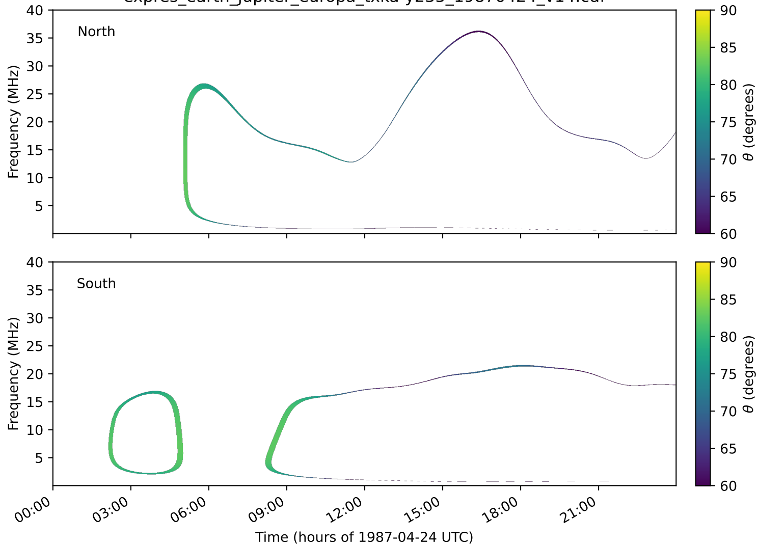
expres_earth_jupiter_europa_txka-y235_19870424_v14.cdf
