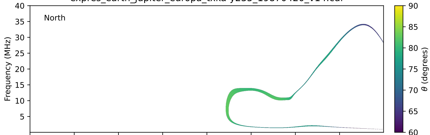
expres_earth_jupiter_europa_txka-y235_19870420_v14.cdf
