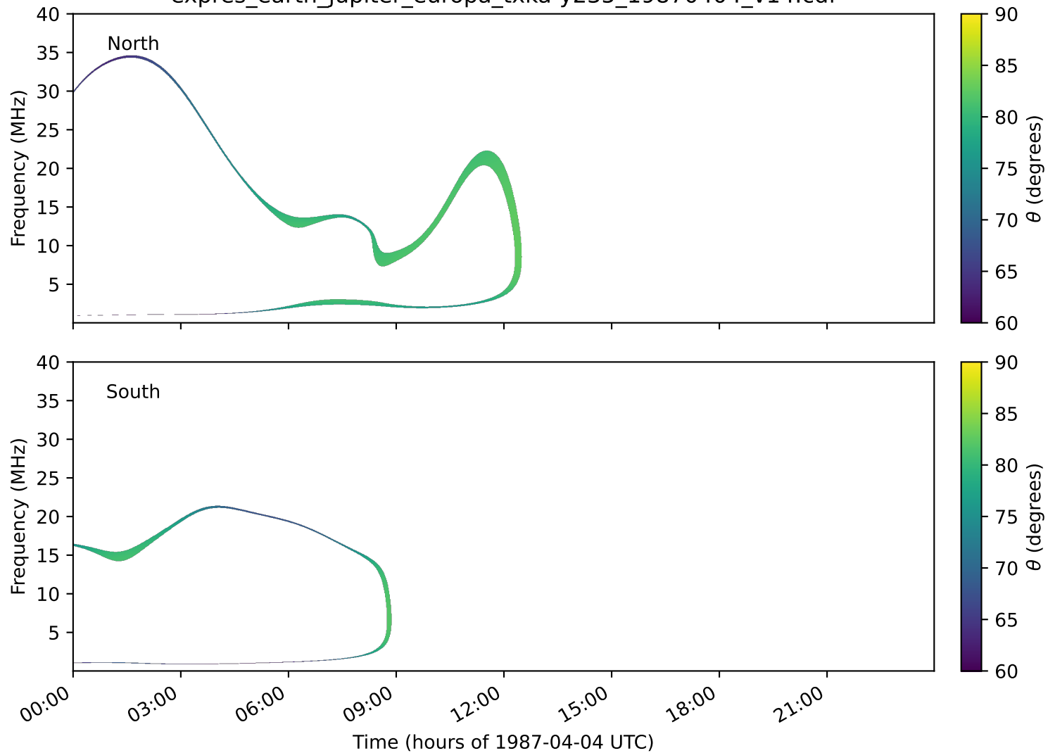
expres_earth_jupiter_europa_txka-y235_19870404_v14.cdf
