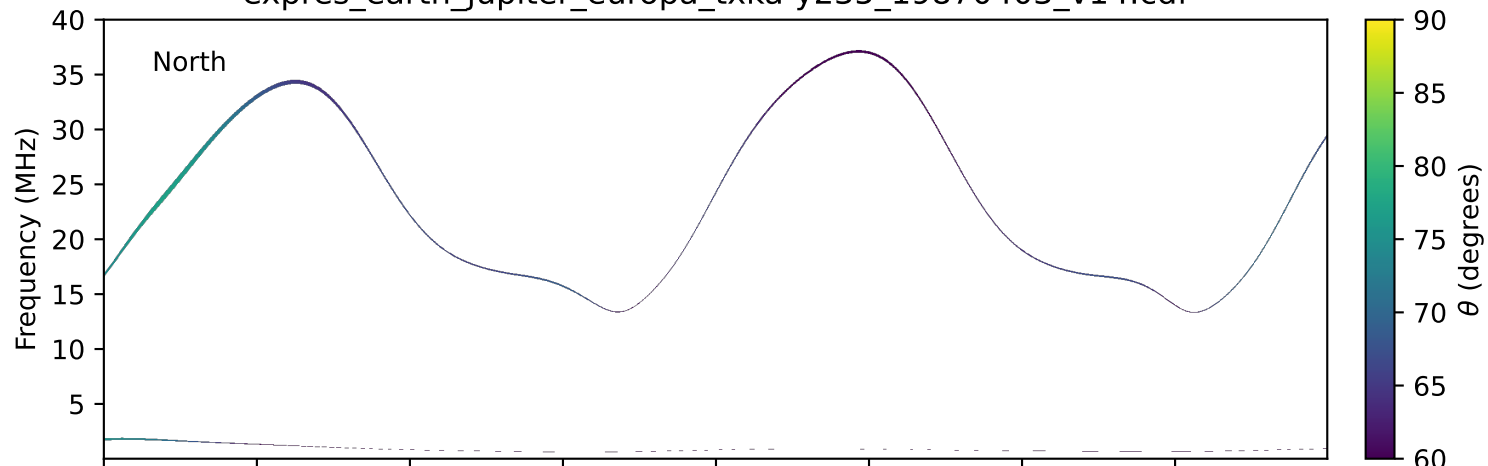
expres_earth_jupiter_europa_txka-y235_19870403_v14.cdf
