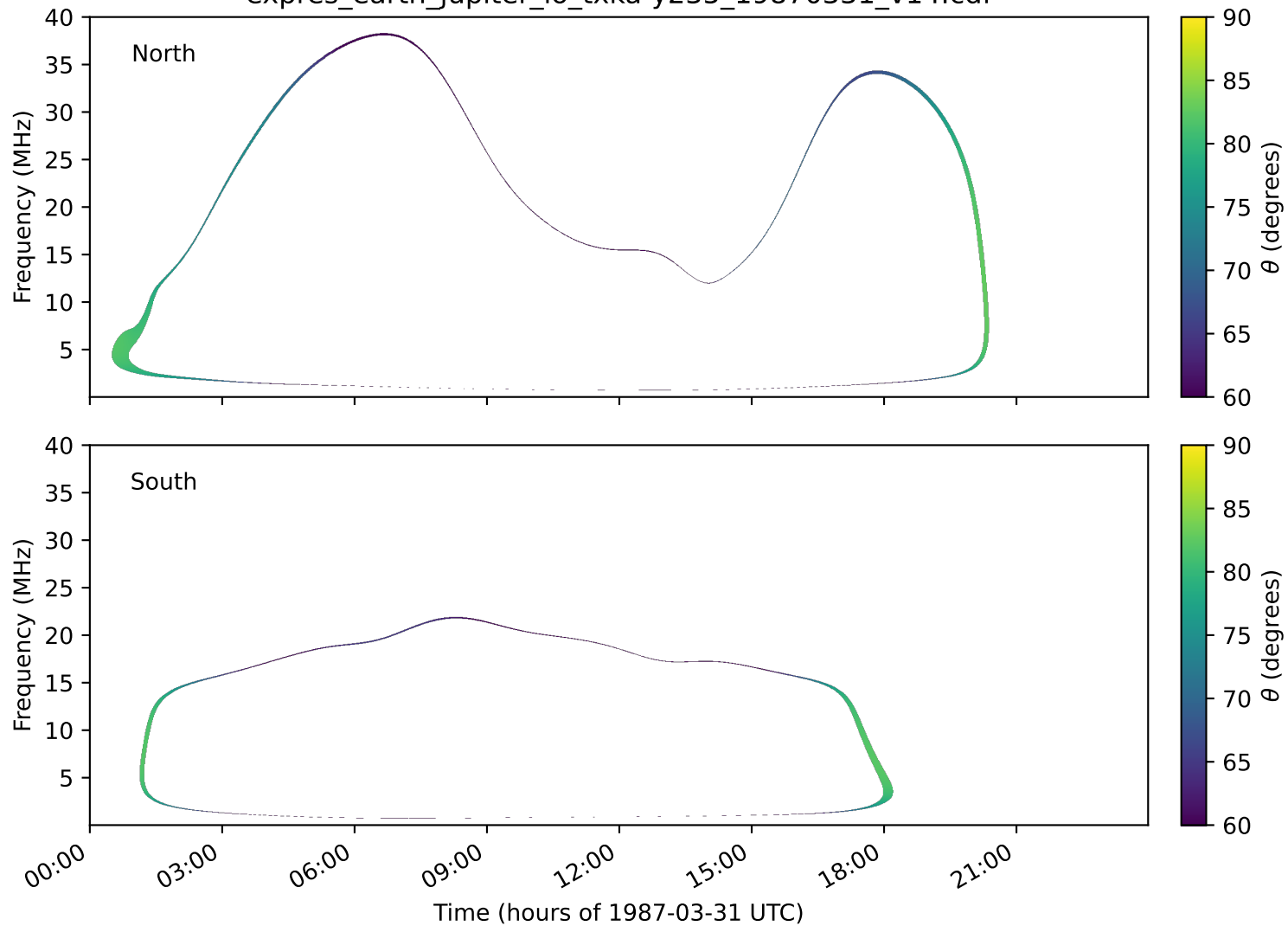
expres_earth_jupiter_io_txka-y235_19870331_v14.cdf
