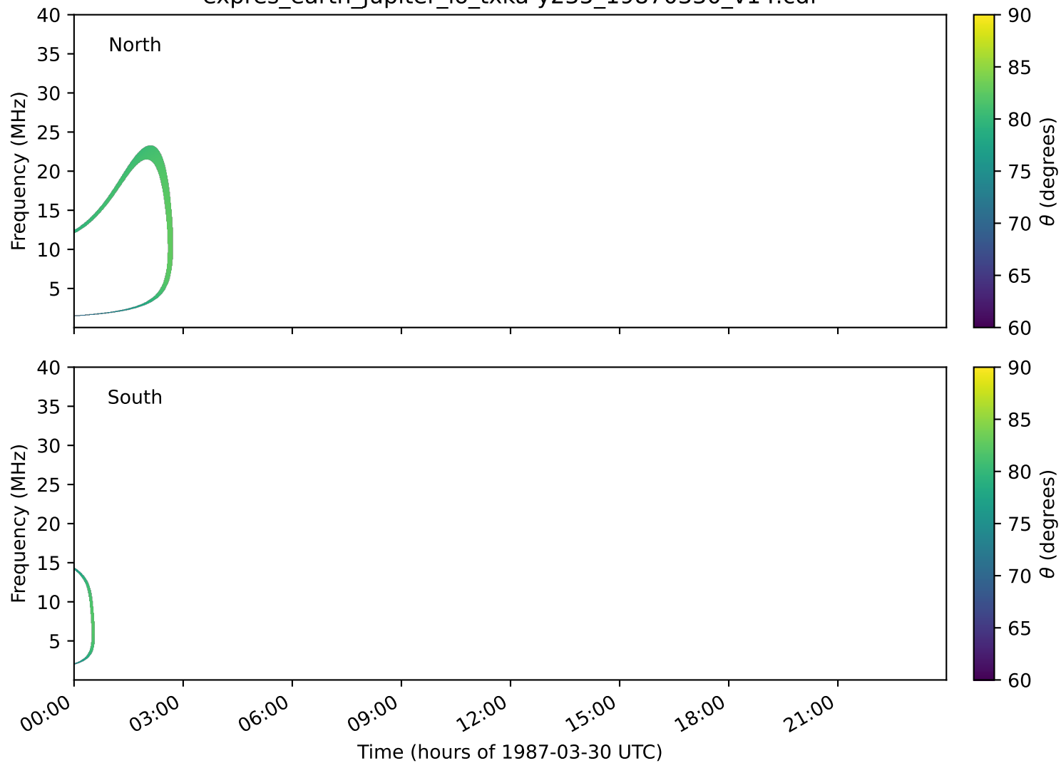
expres_earth_jupiter_io_txka-y235_19870330_v14.cdf
