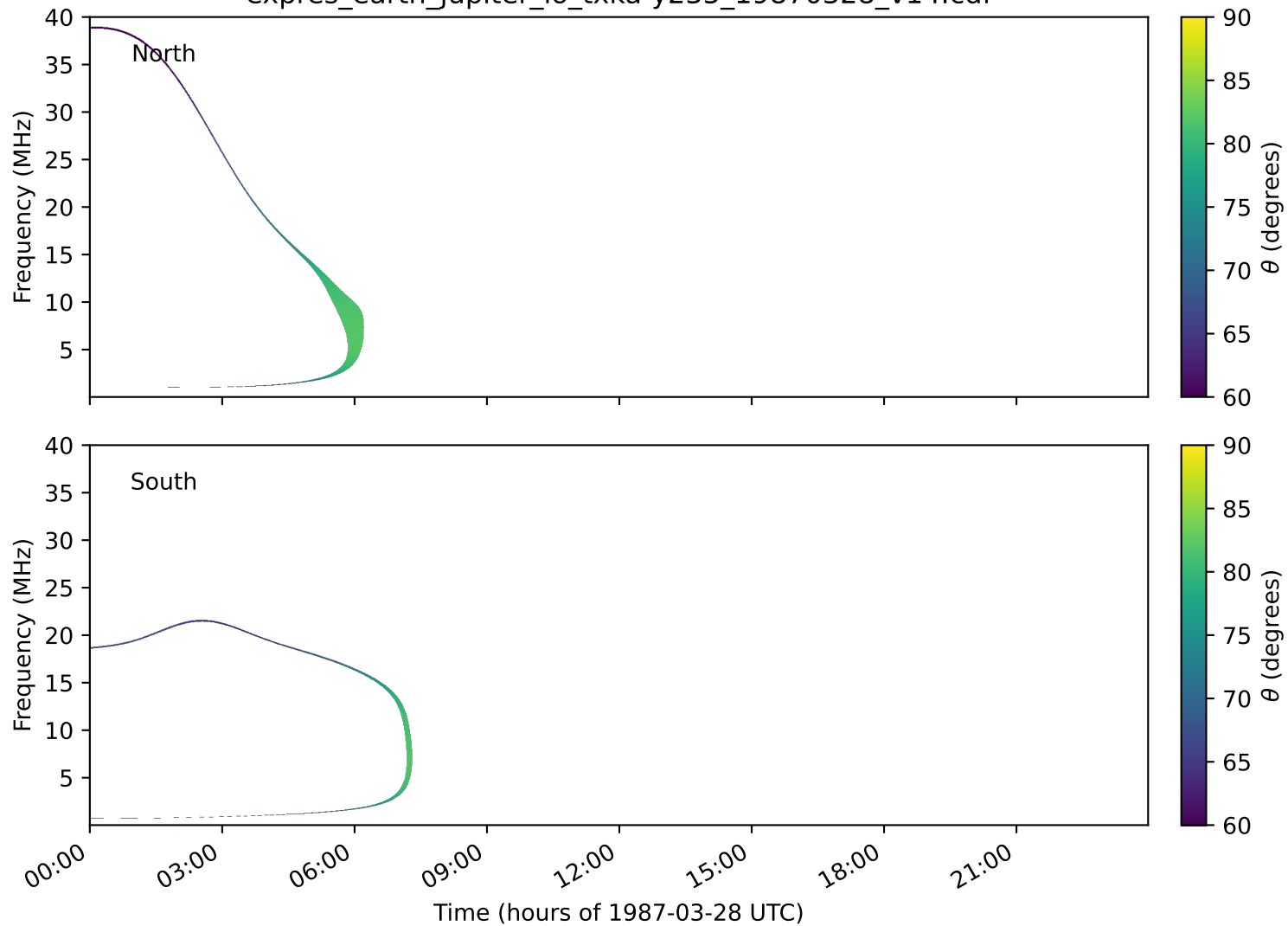
expres_earth_jupiter_io_txka-y235_19870328_v14.cdf
