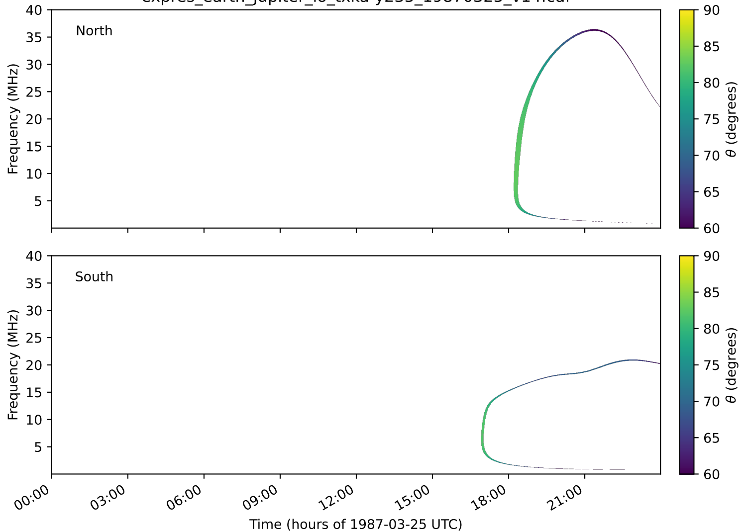
expres_earth_jupiter_io_txka-y235_19870325_v14.cdf
