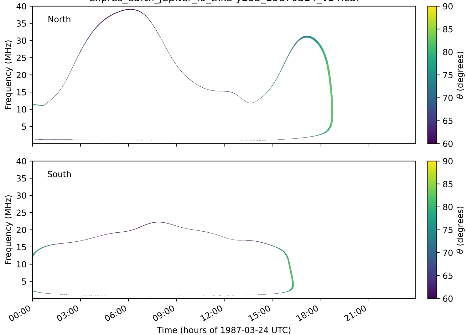
expres_earth_jupiter_io_txka-y235_19870324_v14.cdf
