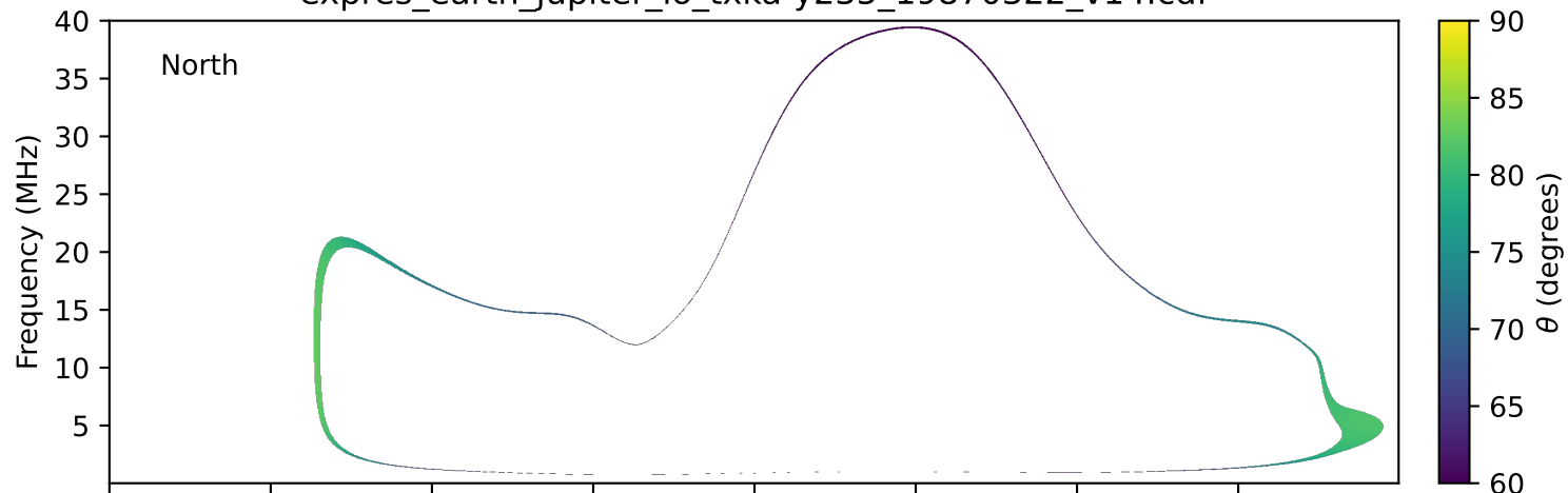
expres_earth_jupiter_io_txka-y235_19870322_v14.cdf
