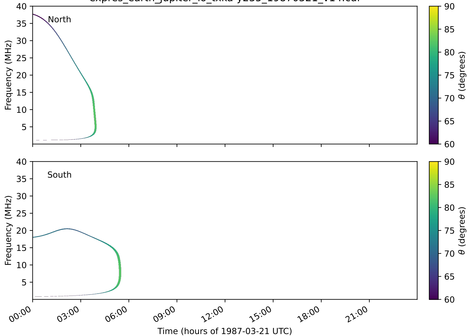
expres_earth_jupiter_io_txka-y235_19870321_v14.cdf
