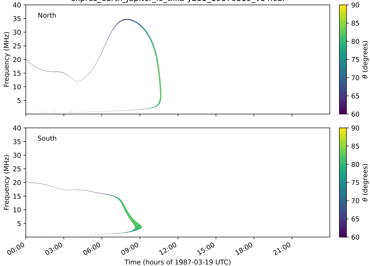
expres_earth_jupiter_io_txka-y235_19870319_v14.cdf
