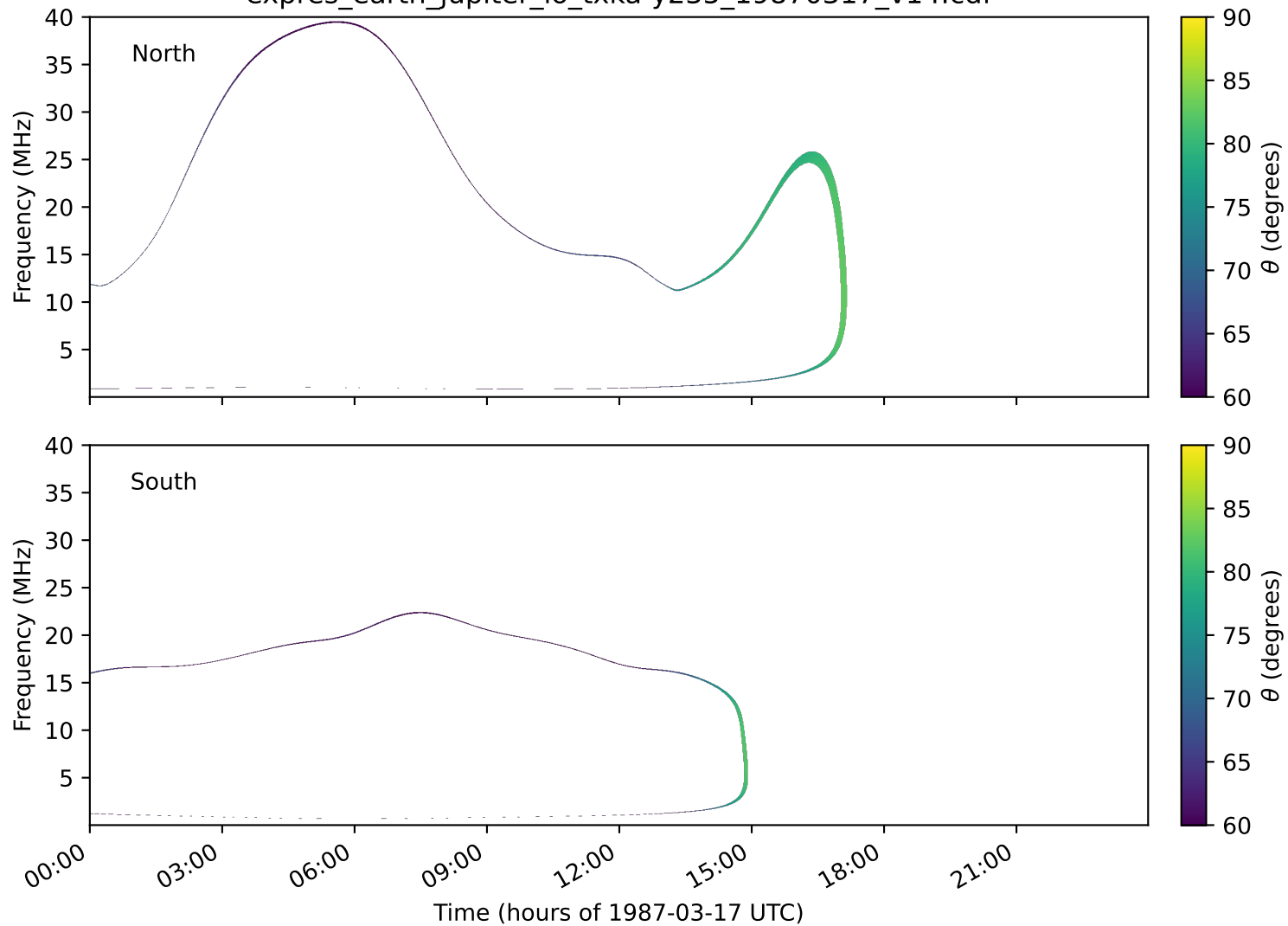
expres_earth_jupiter_io_txka-y235_19870317_v14.cdf
