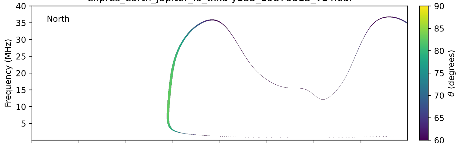
expres_earth_jupiter_io_txka-y235_19870313_v14.cdf
