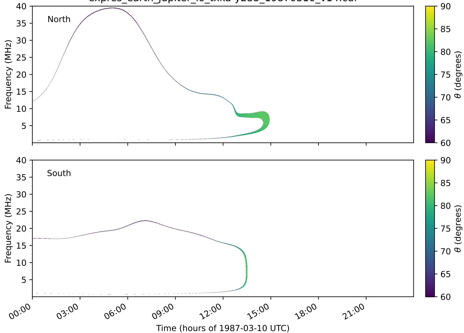
expres_earth_jupiter_io_txka-y235_19870310_v14.cdf
