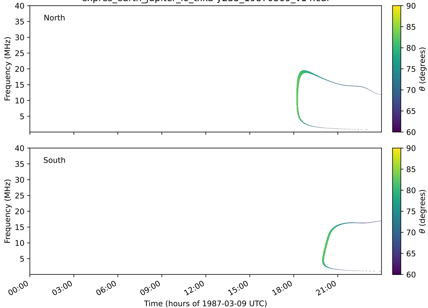
expres_earth_jupiter_io_txka-y235_19870309_v14.cdf
