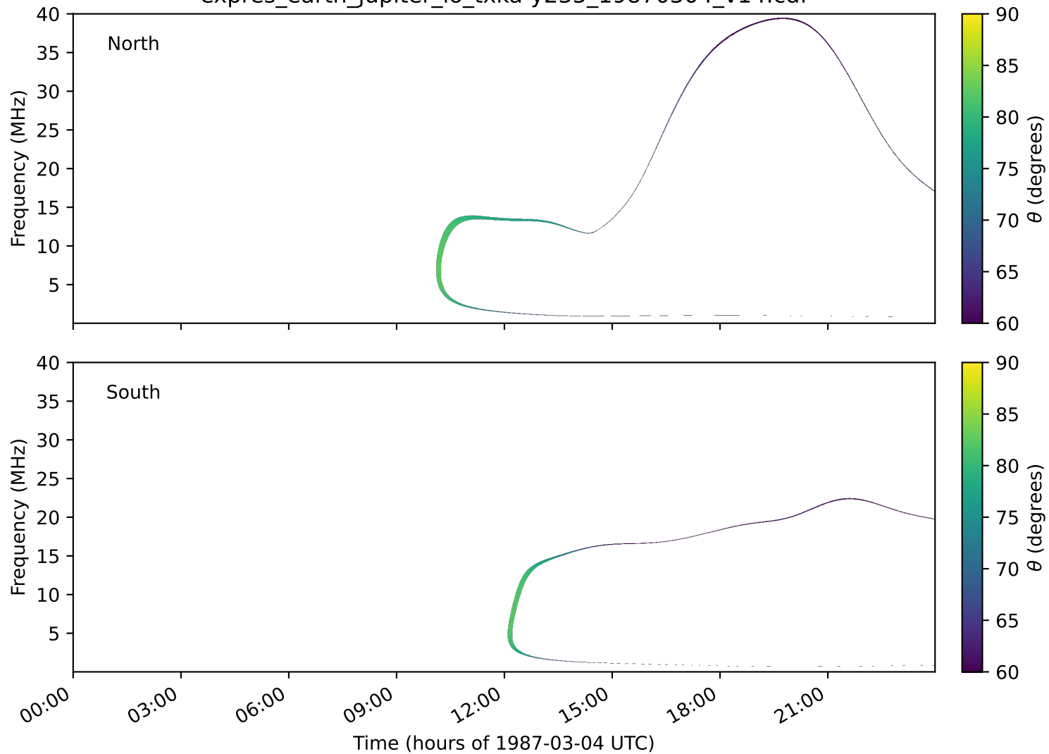
expres_earth_jupiter_io_txka-y235_19870304_v14.cdf
