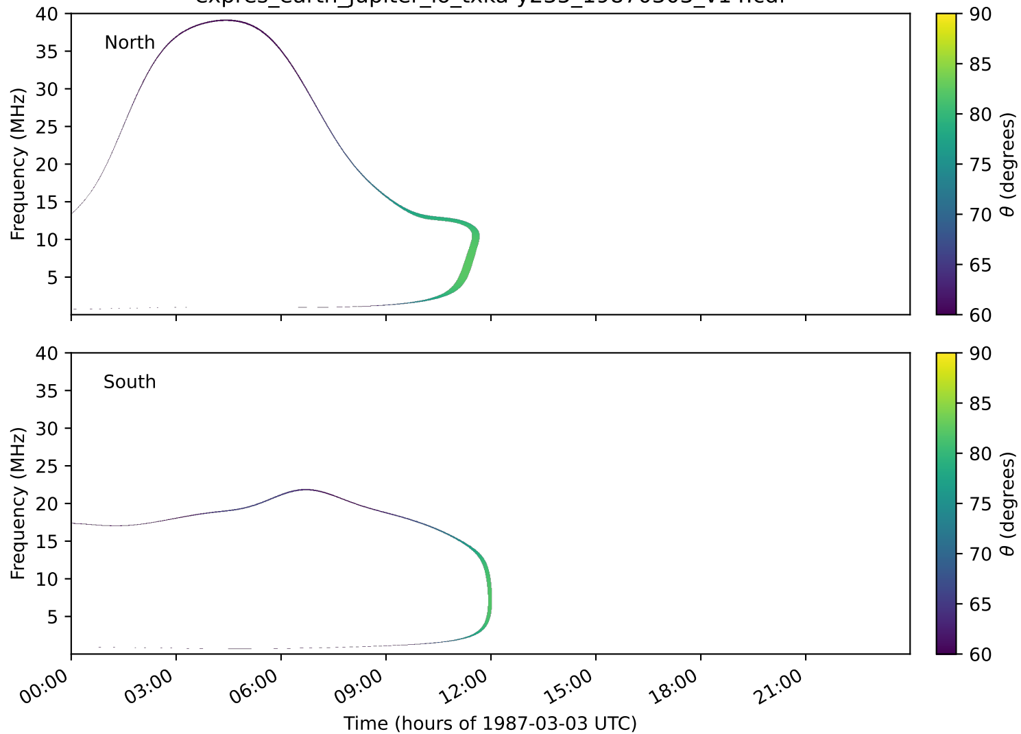
expres_earth_jupiter_io_txka-y235_19870303_v14.cdf
