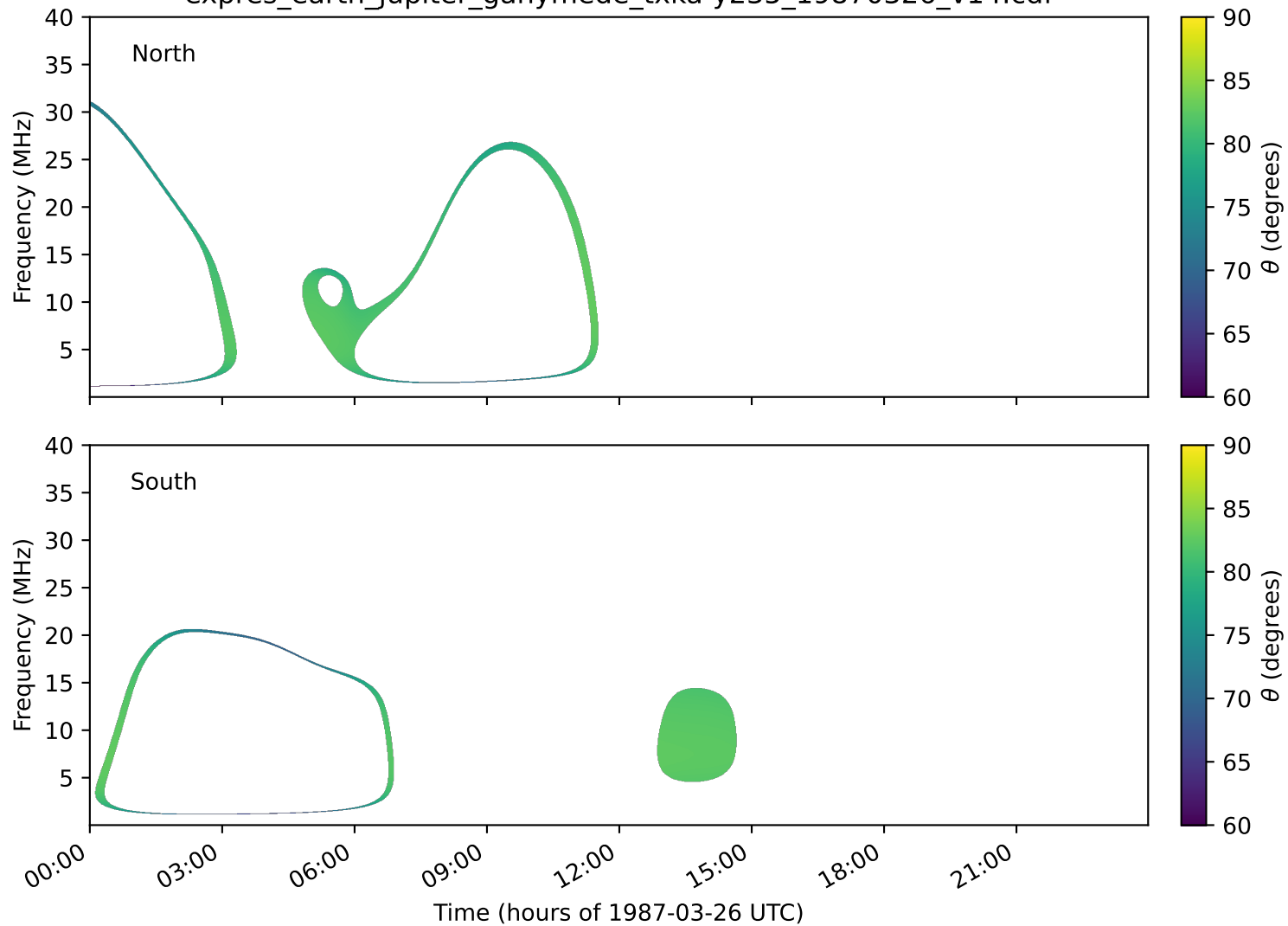
expres_earth_jupiter_ganymede_txka-y235_19870326_v14.cdf
