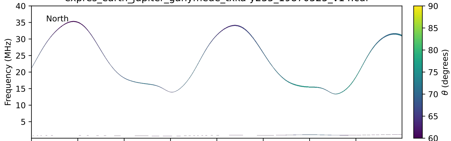
expres_earth_jupiter_ganymede_txka-y235_19870325_v14.cdf
