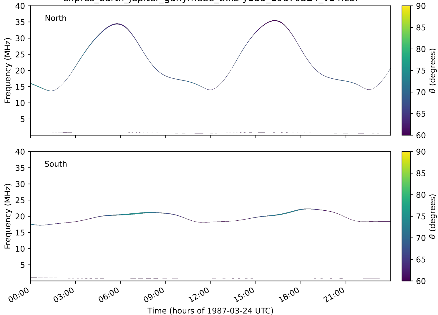
expres_earth_jupiter_ganymede_txka-y235_19870324_v14.cdf
