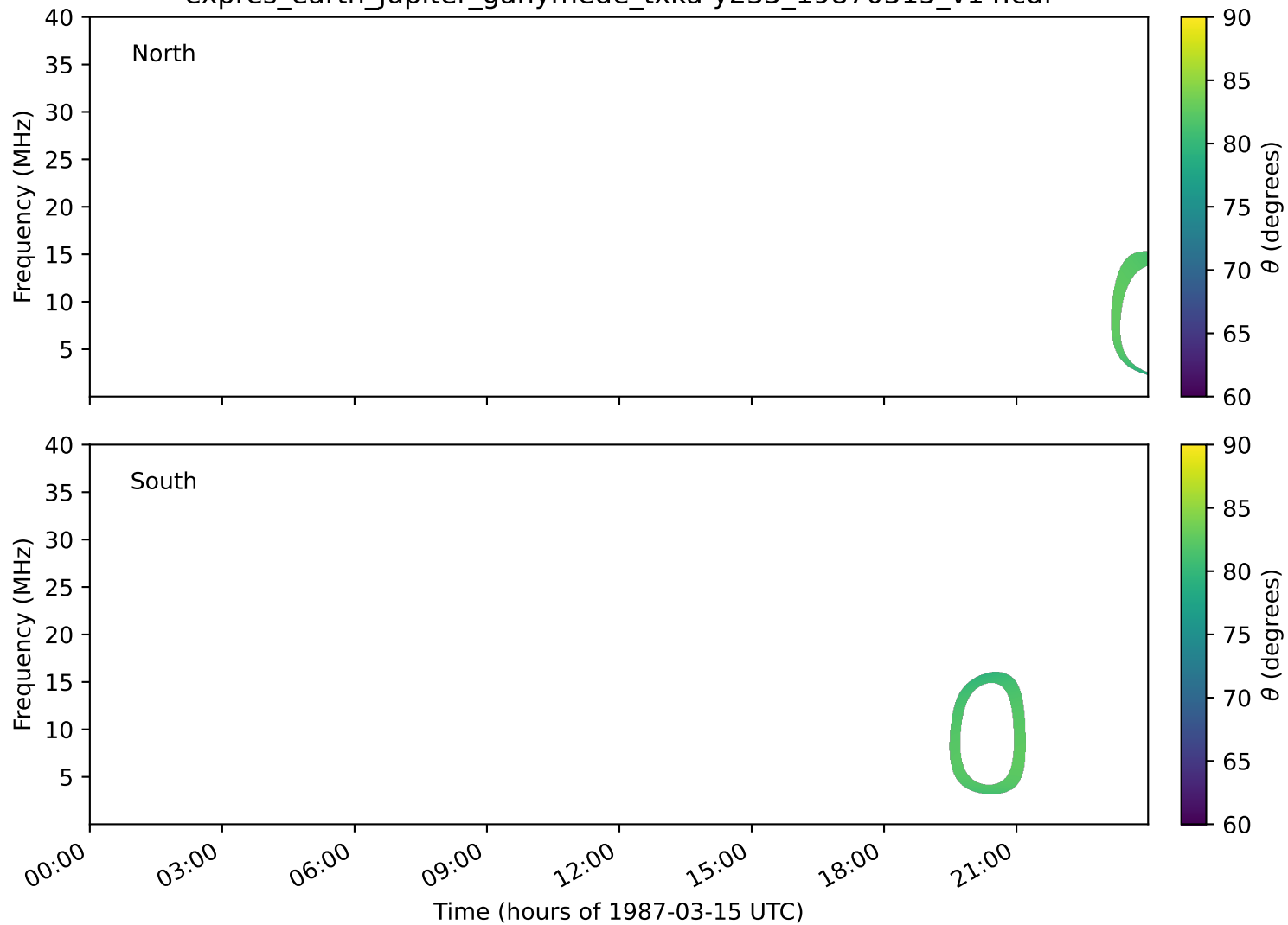
expres_earth_jupiter_ganymede_txka-y235_19870315_v14.cdf
