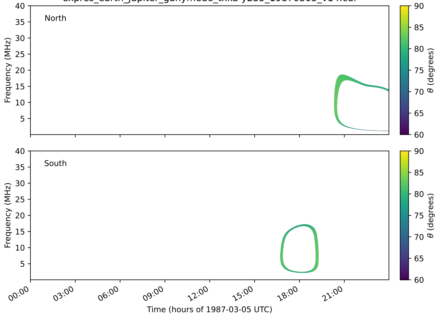
expres_earth_jupiter_ganymede_txka-y235_19870305_v14.cdf
