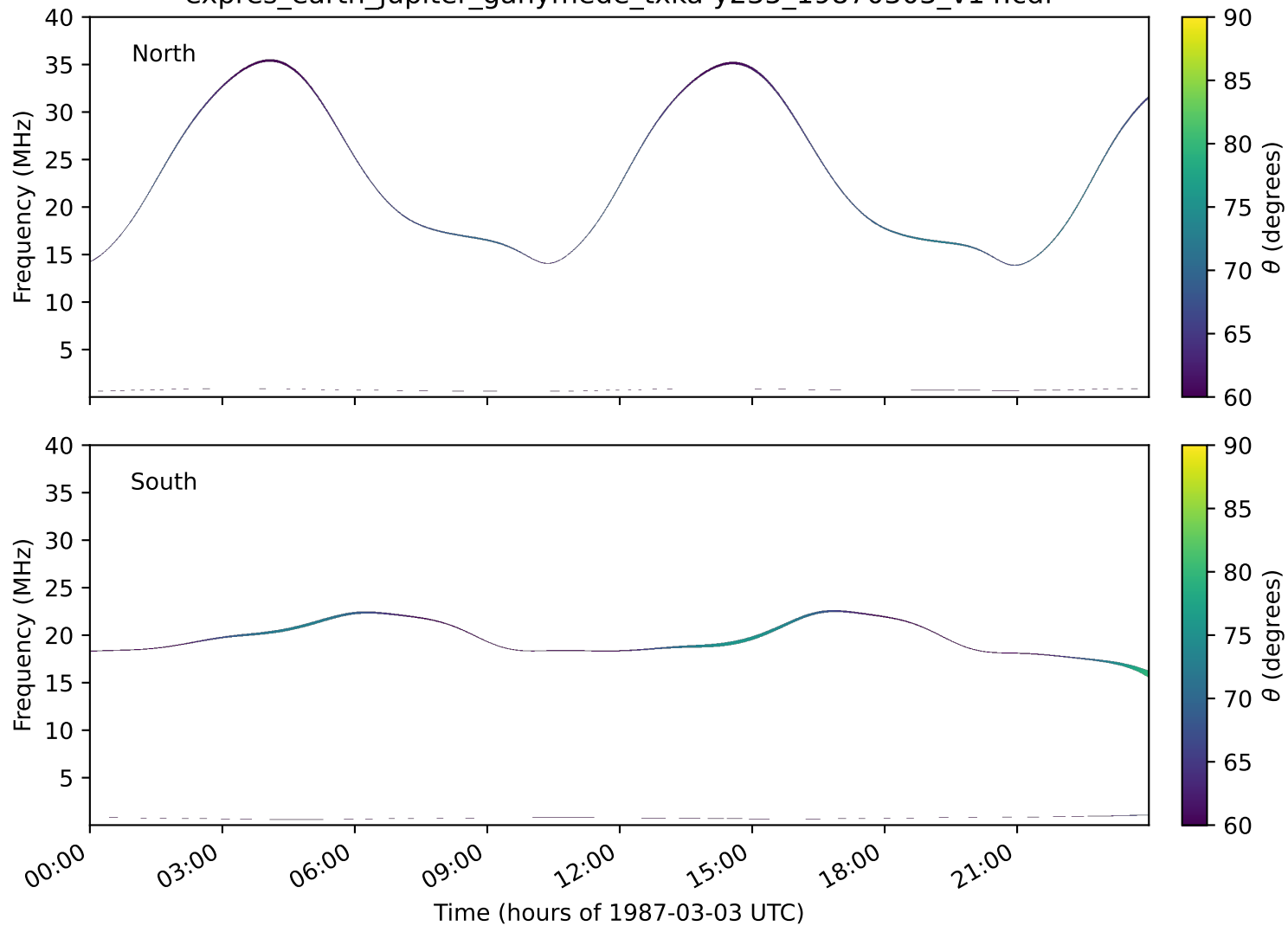
expres_earth_jupiter_ganymede_txka-y235_19870303_v14.cdf
