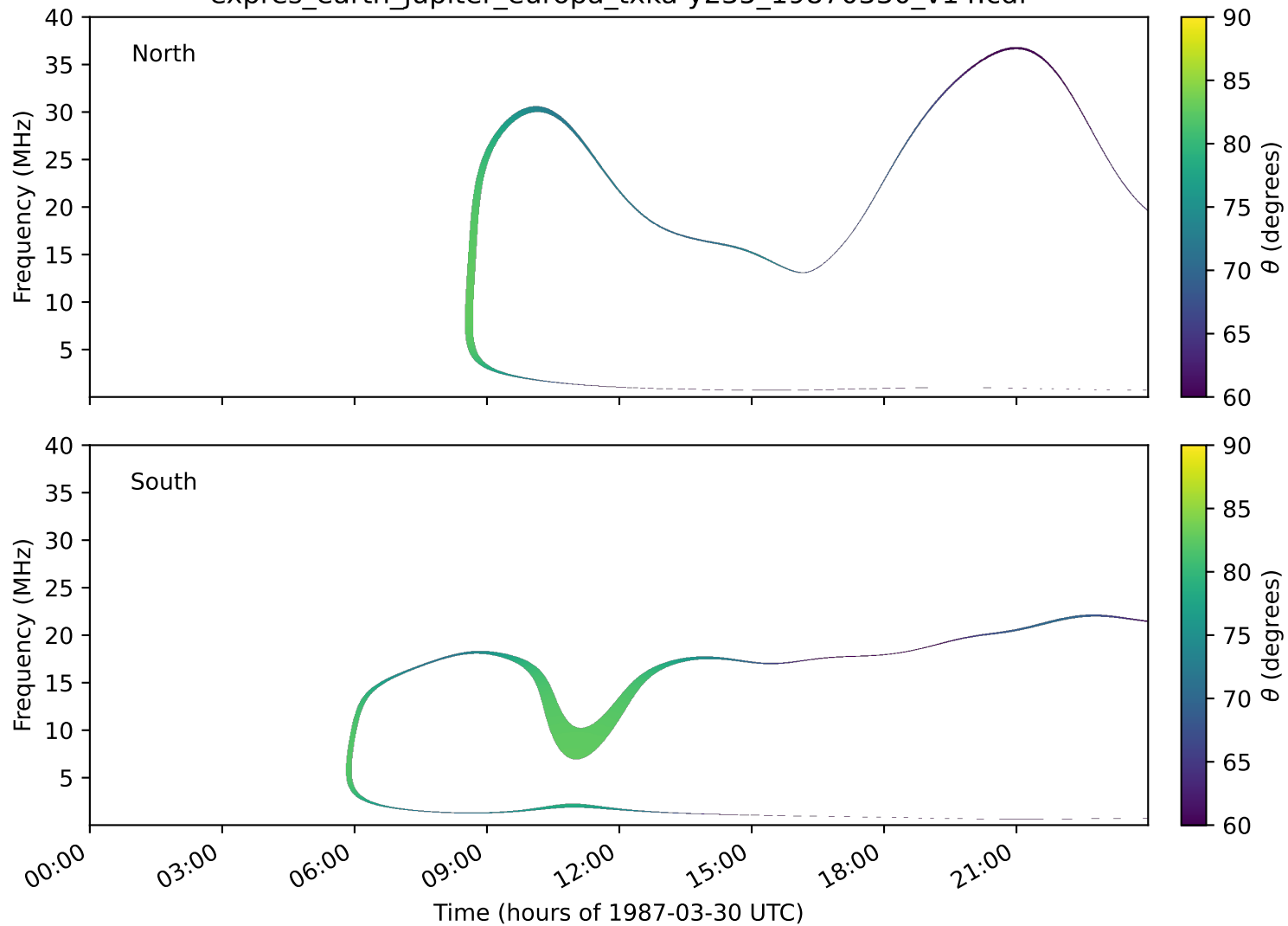
expres_earth_jupiter_europa_txka-y235_19870330_v14.cdf
