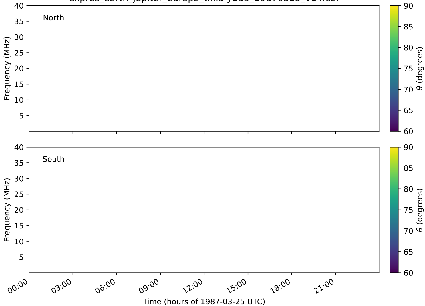
expres_earth_jupiter_europa_txka-y235_19870325_v14.cdf
