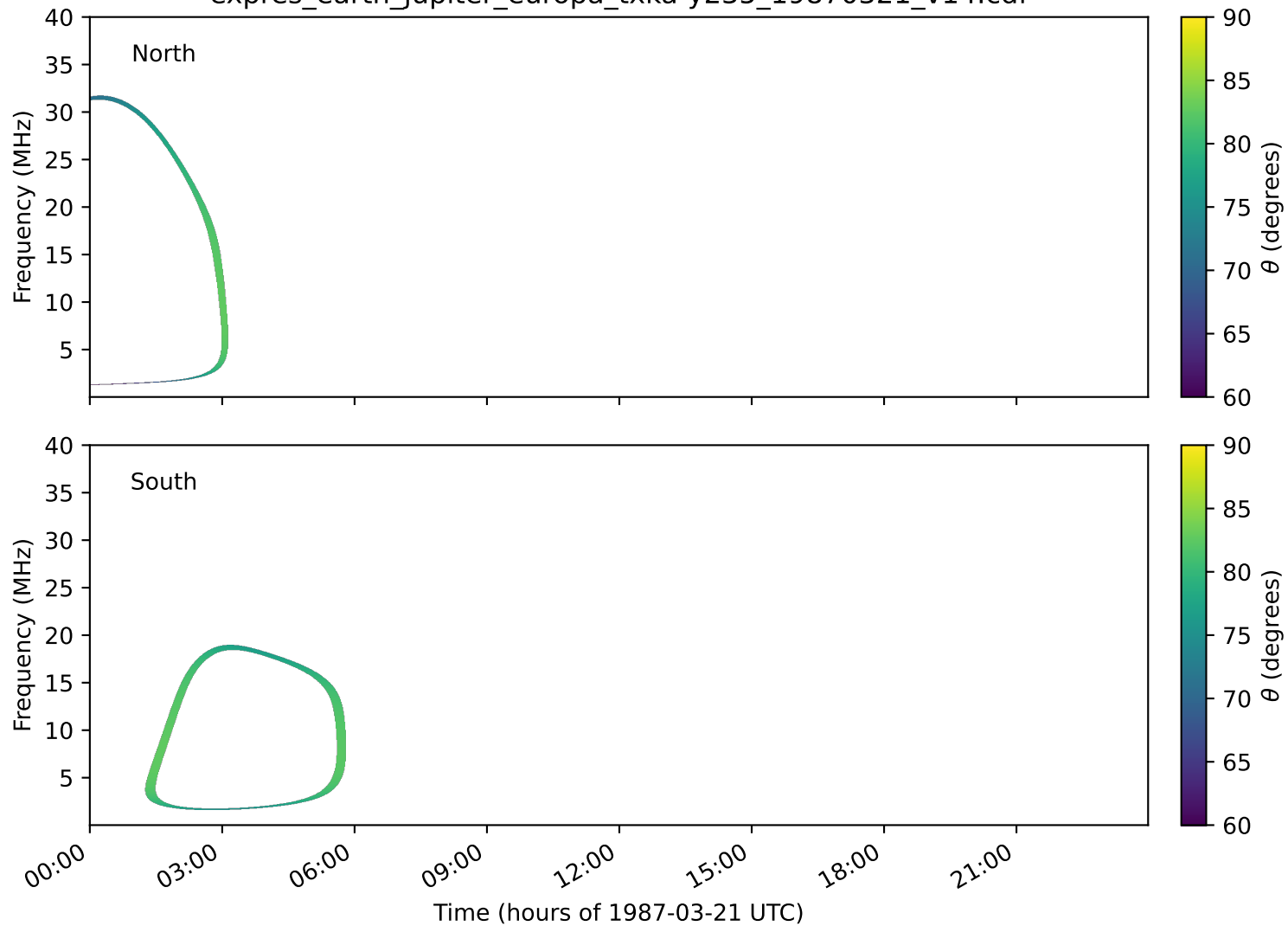
expres_earth_jupiter_europa_txka-y235_19870321_v14.cdf
